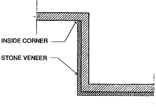
CORRECT USE OF NATURAL STONE VENEER MATERIAL ENDS AT AN INSIDE CORNER.
